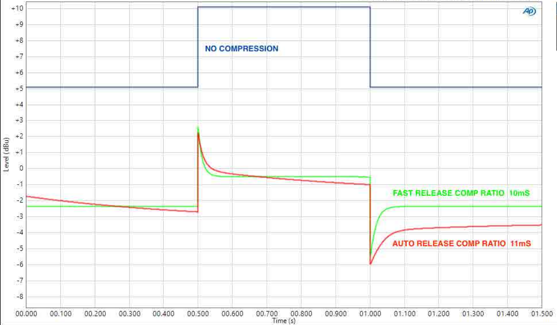
Daking Comp II Release Times with 1kHz Input
